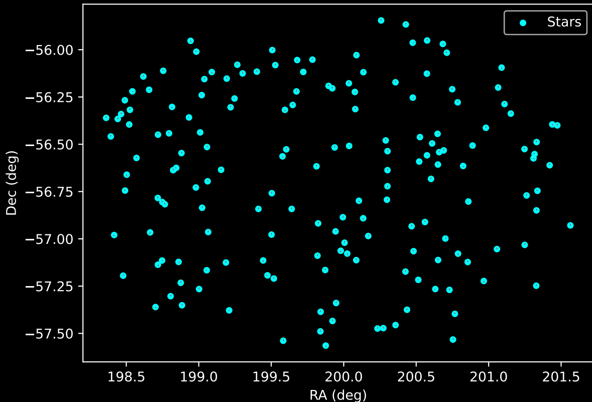
APOGEE DR17 Field: [266-24-O_TESS] Proper Motion Vectors for Gaia Star Field (n= 166)
