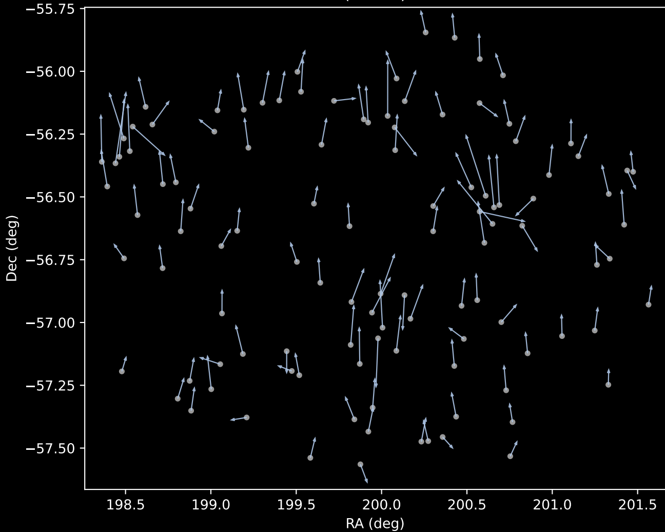
APOGEE DR17 Cluster 1 Proper Motion Vectors (n=111)
