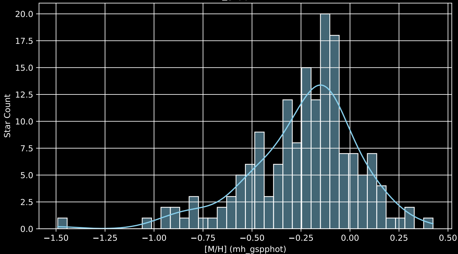
APOGEE DR17 Field: [266-24-O_TESS [M/H] (mh_gspphot) (n= 166)
