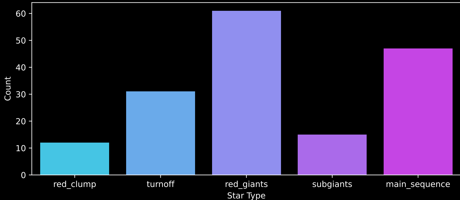
APOGEE DR17 Field: [266-24-O_TESS] Count plot of Star Type
