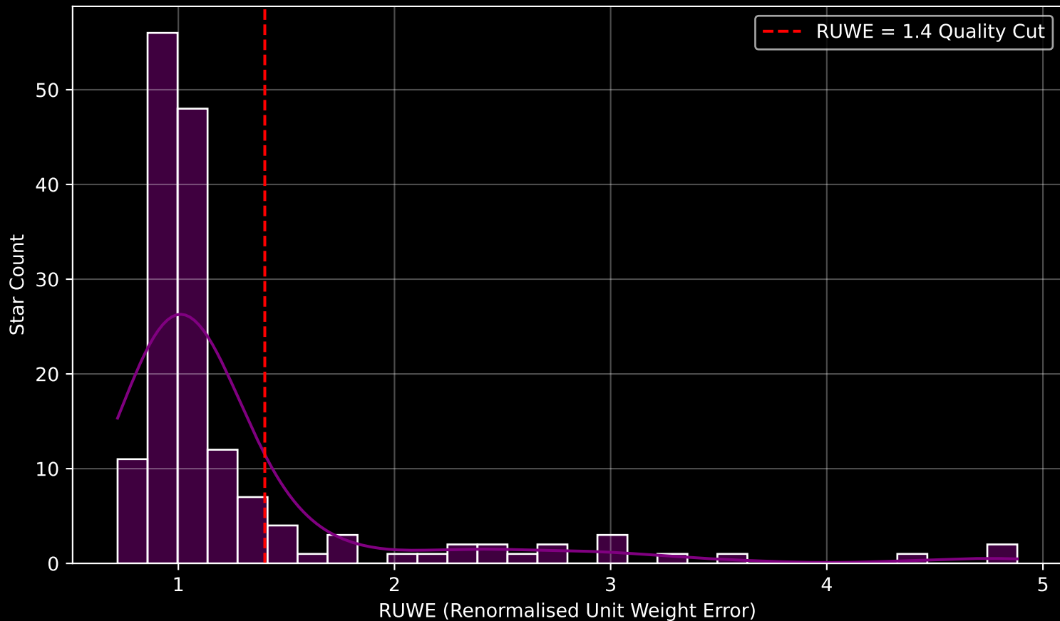
GAPOGEE DR17 Field [266-24-O_TESS] RUWE Distribution (n= 159)
