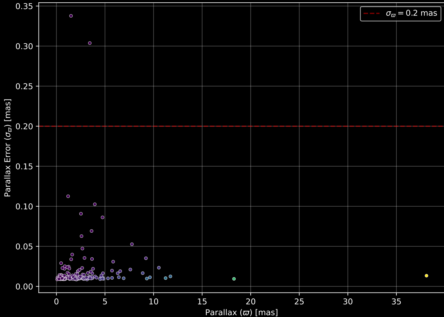
APOGEE DR17 Field: [266-24-O_TESS] Parallax Quality (n= 166)
