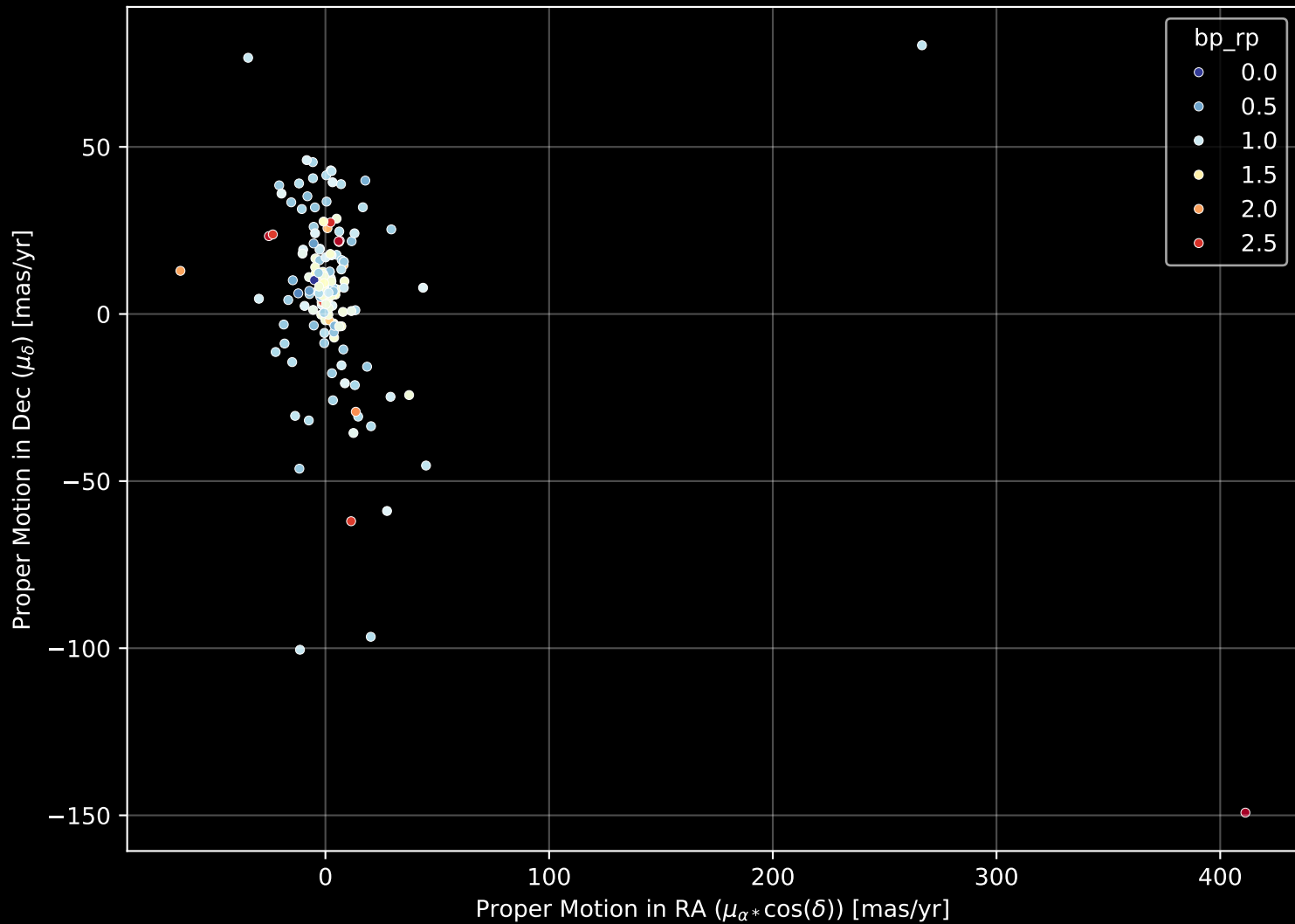
APOGEE DR17 Field: [266-24-O_TESS] Proper Motion Diagram (n= 166)
